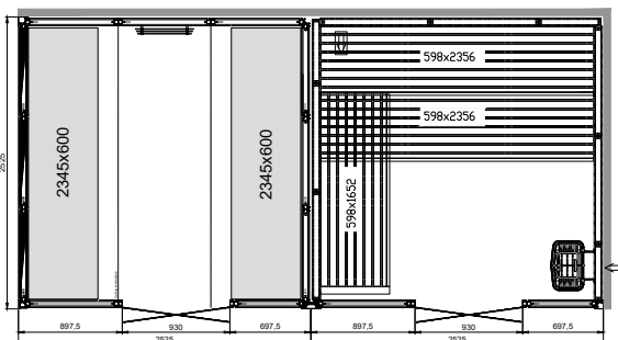
PANACEA TWIN 2121 WD
