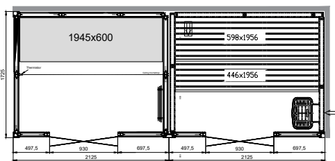
PANACEA TWIN 2117 WD
